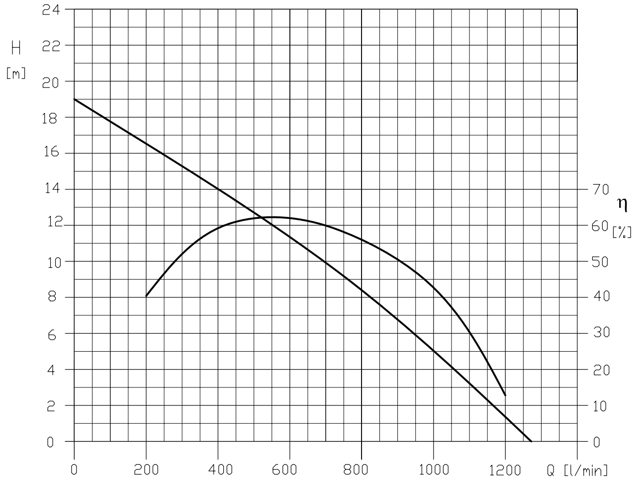
DUMPER 2X 52.2-S
