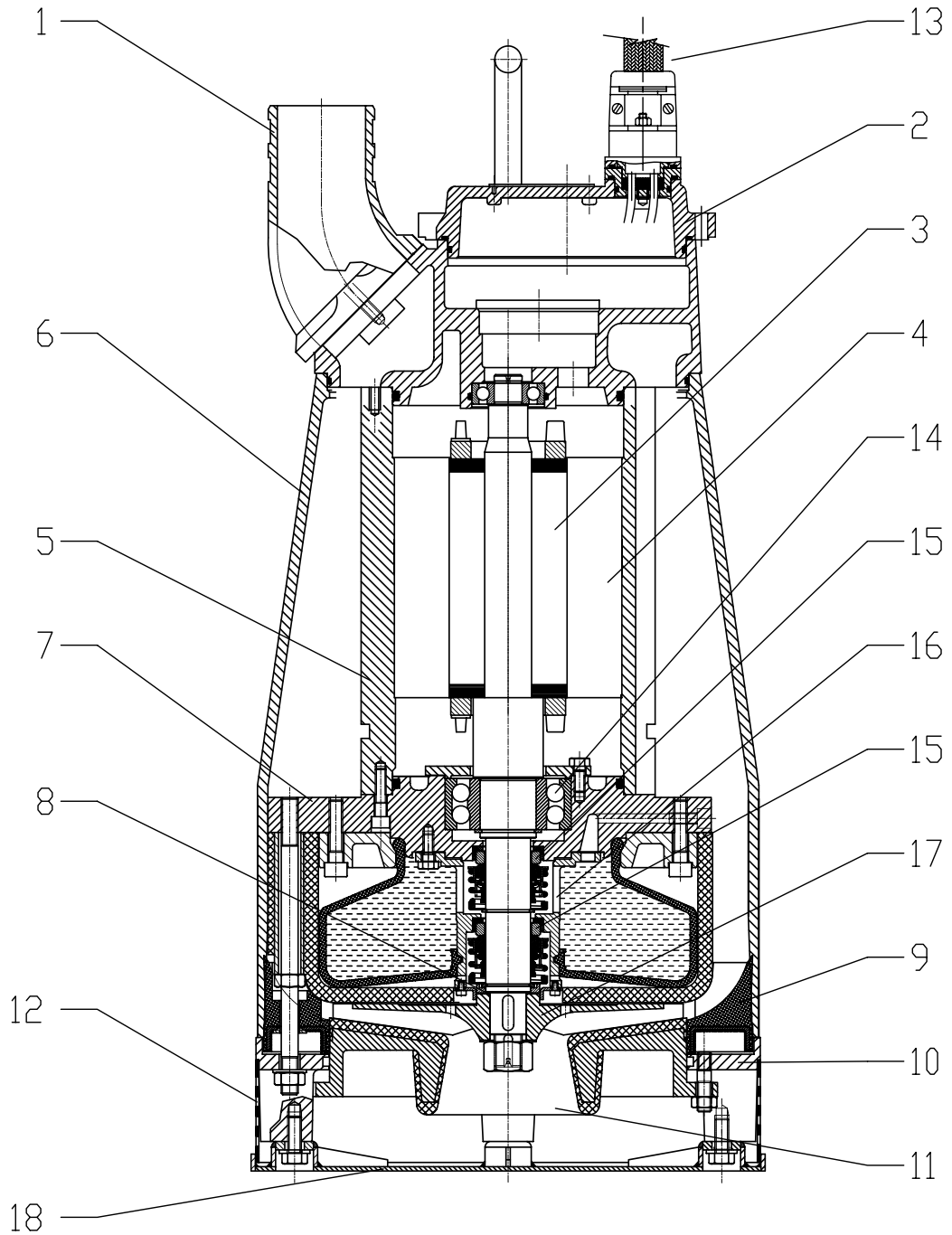
SECTIONAL VIEW DUMPER 5X 58-S
